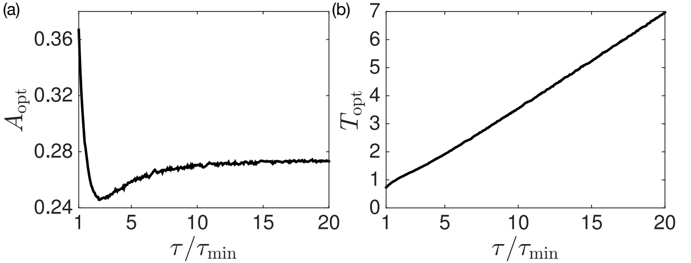
Figure S1: Optimized values of the parameters A and T appearing in the function f(t) Eq. (S4) as a function of \tau/\tau_{\min} for t_i = -t_f .
