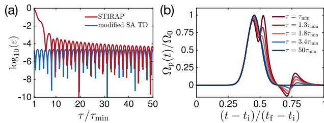
FIG. 3. (a) Comparison of the residual error for STIRAP with Gaussian densities [Eq. (23)] and the modified SATD [Eq. (24)] as a function of the effective protocol duration \tau in units of \tau_{\min} . The residual error is reduced by several orders of magnitude in the nonadiabatic regime. (b) Corrected pump pulse for different values of \tau as a function of time (t - t_i) in units of the total protocol time (t_f - t_i) .
