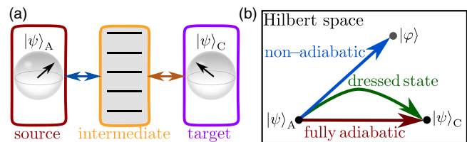
FIG. 1. (a) Schematic of a composite quantum system where the source and the target systems (qubits in this schematic) are coupled via some intermediate system. (b) Schematic of the possible evolutions: (red line) perfect adiabatic evolution; (blue line) speeding up the evolution results in nonadiabatic errors leading to an imperfect state transfer; (green line) by dressing the adiabatic eigenstates it is possible to design an evolution that leads to a perfect state transfer.
