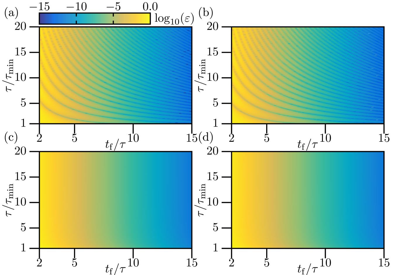
Figure S2: Error \varepsilon = 1 - F Eq. (S11) as a function of the normalized effective protocol time \tau/\tau_{\min} and normalized final time t_f/\tau (we chose t_f = -t_i ) for the Vitanov style corrected pulses : (a) with SA-TD correction, and (b) with modified SA-TD correction. Upper bound for the error \varepsilon_{\max} = 1 - F_{\min} Eq. (S12) : (c) with SA-TD correction, and (d) with modified SA-TD correction.
