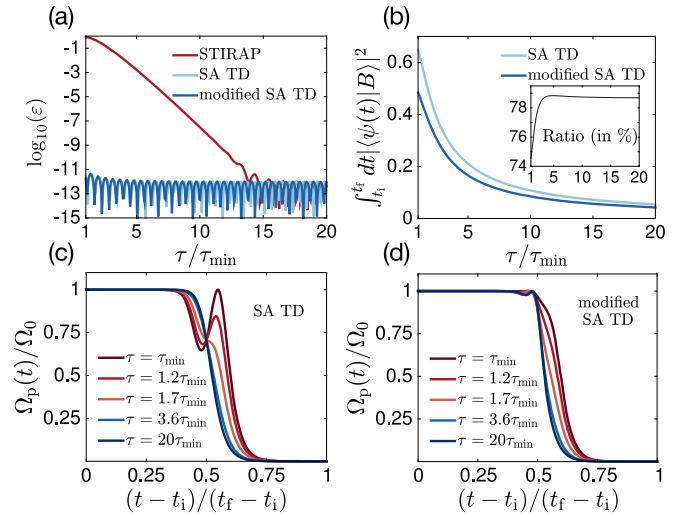
FIG. 2. (a) Comparison of the residual error between STIRAP [Eq. (19)], SATD [Eq. (20)], and the modified SATD [Eq. (21)] as a function of the effective protocol duration \tau in units of \tau_{\min} . (b) Comparison of the integrated population in |B\rangle over the whole protocol time between SATD [Eq. (20)] and our new dressed state approach [Eq. (21)] as a function of \tau in units of \tau_{\min} . Inset: ratio of those two quantities. The integrated population is reduced by at least 21% and at most 26% with our new protocol. Plot of the corrected pump pulse for SATD (c) and the modified SATD (d) for different values of \tau as a function of time (t - t_i) in units of the total protocol time (t_f - t_i) .
