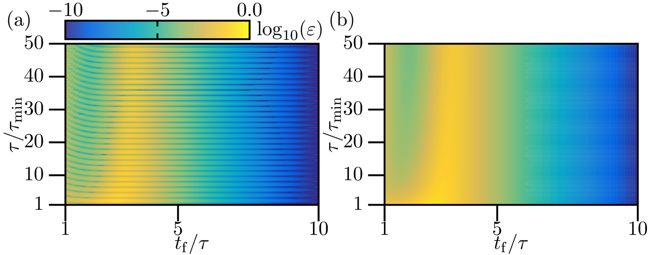
Figure S3: (a) Error \varepsilon = 1 - F Eq. (S11) as a function of the normalized effective protocol time \tau/\tau_{\min} and the normalized final time t_f/\tau (we chose t_f = -t_i ) for the Gaussian corrected pulses. (b) Upper bound for the error \varepsilon_{\max} = 1 - F_{\min} Eq. (S12) for the Gaussian pulses.
